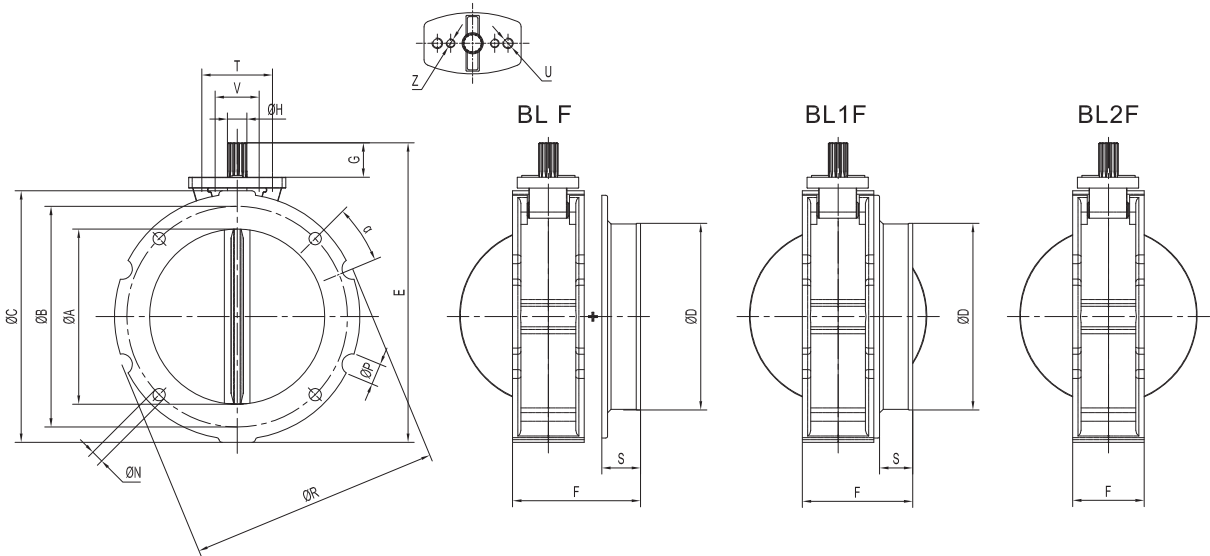
Detachable open type single flange (double flange with single flange)
